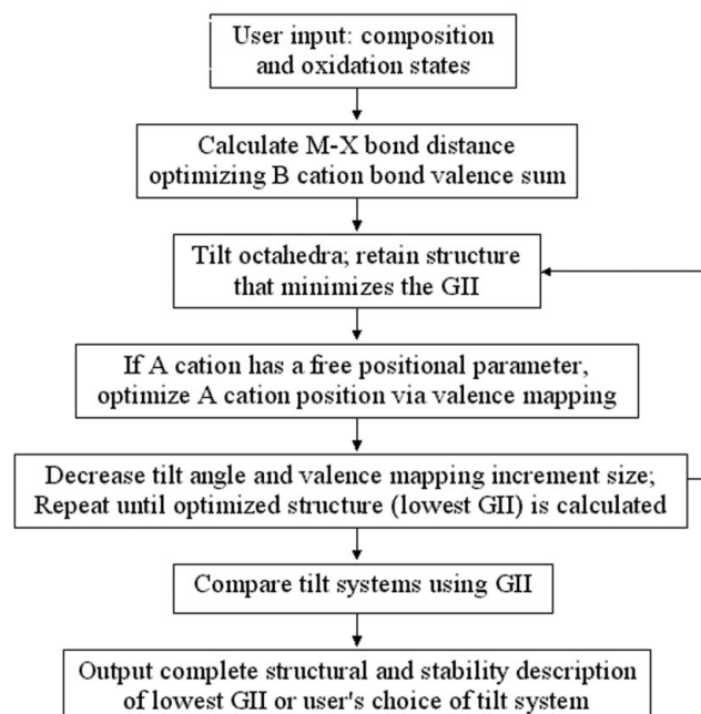
Figure 3 SPuDS operational flowchart.
