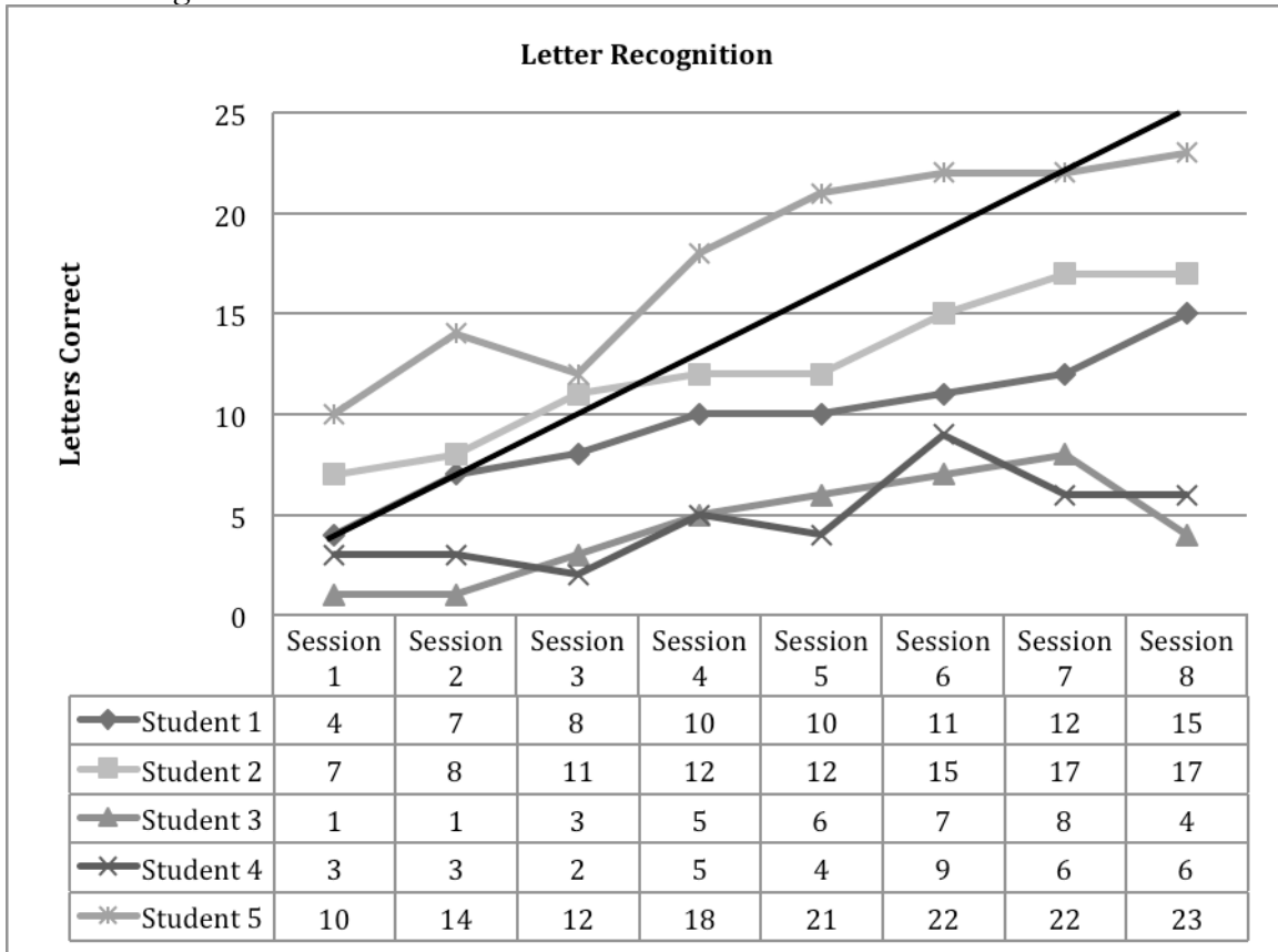
Figure 2. Letter Recognition
