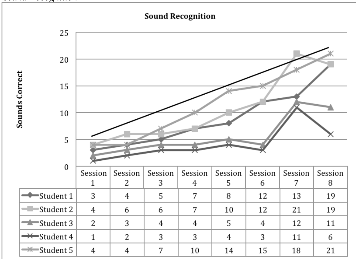
Figure 3. Sound Recognition
